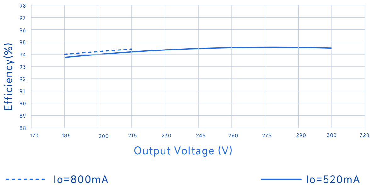
Efficiency Vs. O/P Voltage (Vin=277Vac)
